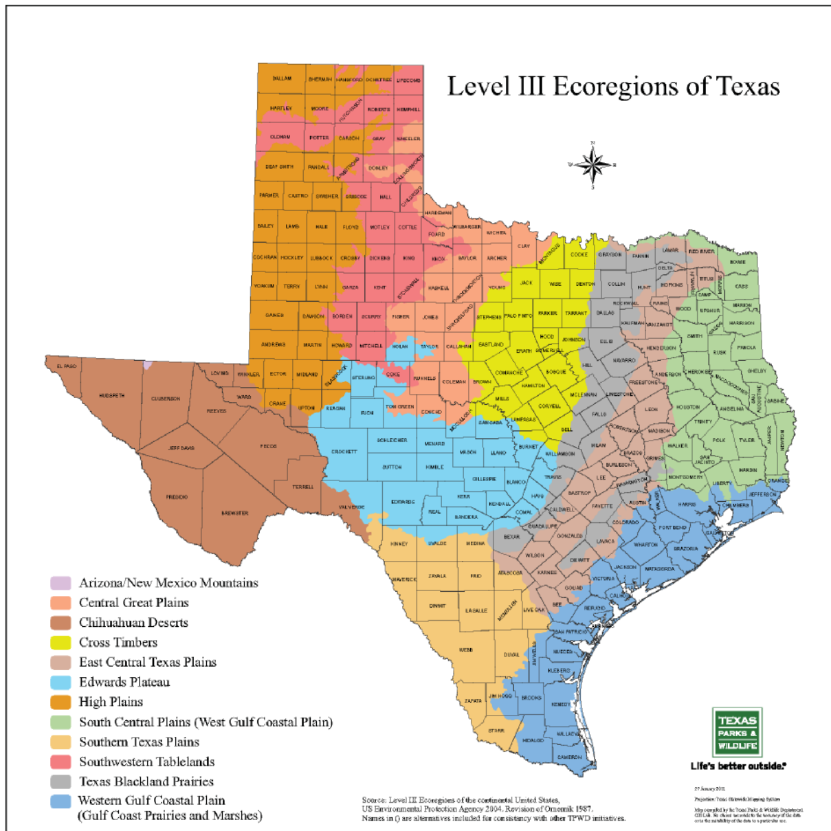
Figure 50: TPWD Ecoregions
