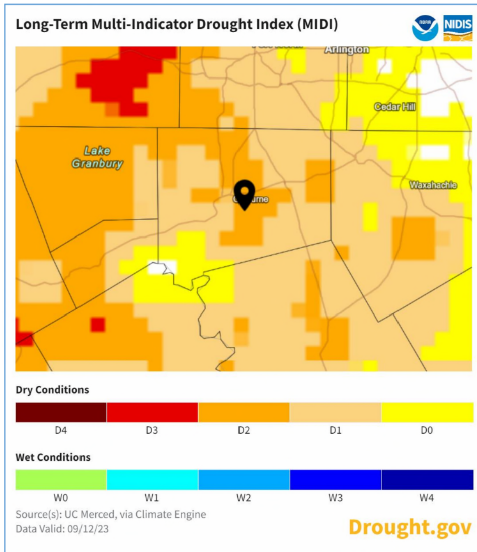
Figure 4: Long-Term MIDI 8
